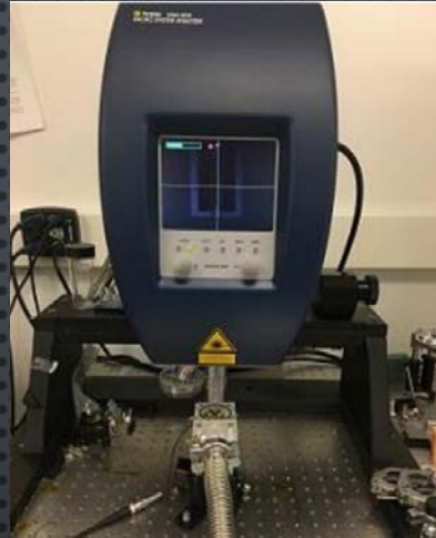
LASER DOPPLER VIBROMETRY (POLYTEC MSA-500)
