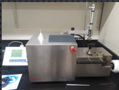
TWIN SCREW EXTRUDER (HAAKE MINILAB II) - POLYMER & NANOCOMPOSITE COMPOUNDER
